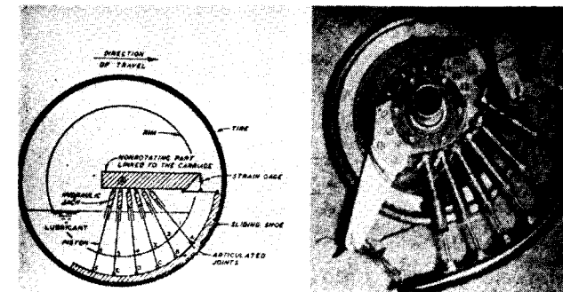
"Schematic and internal view of experimental wheel." (Army R&D August-September 1969)
