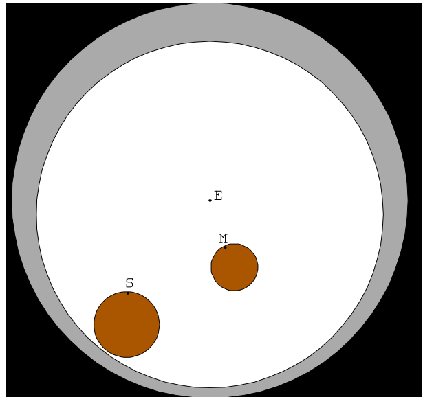
Ptolemaic spheres.
