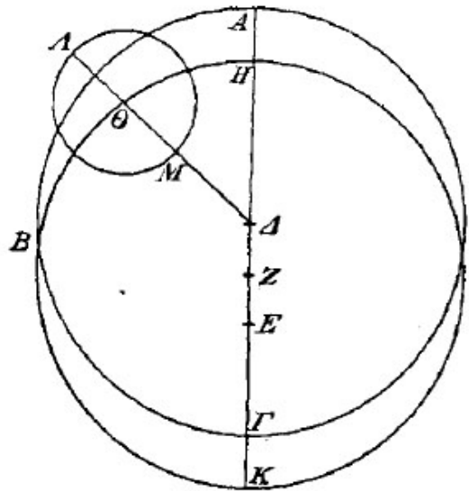
The equant model [Heiberg 1897; II, 254]
