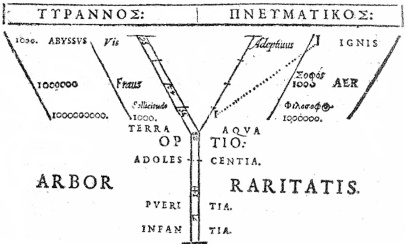
The tree of rarity
