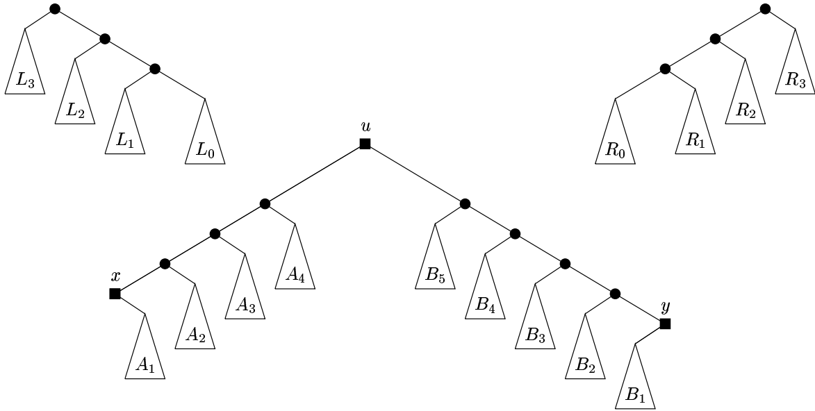
Figure 5: The trees L , T' , and R
